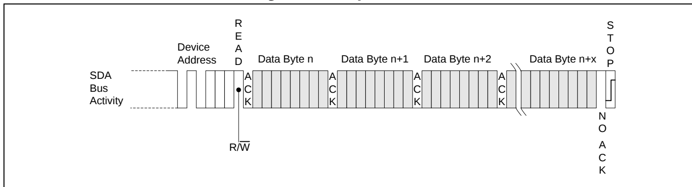
Figure 5-10. Sequential Read
