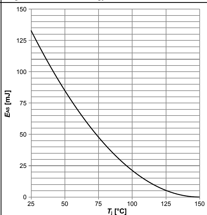
Diagram 16: Avalanche energy
