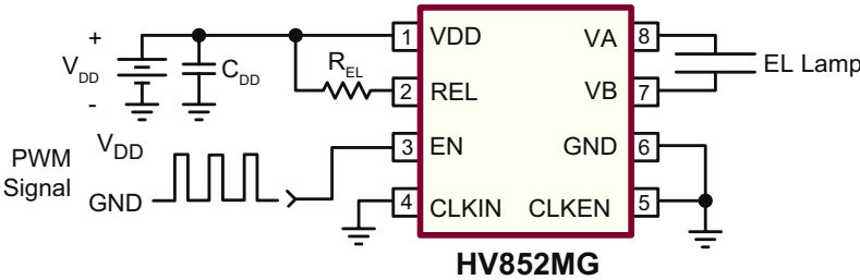
Figure 4: PWM Dimming Circuit
