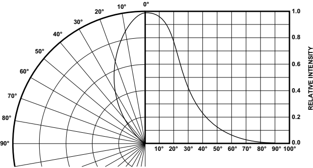
Figure 5: Relative Luminous Intensity vs. Angular Displacement for T-1¼ Lamp
