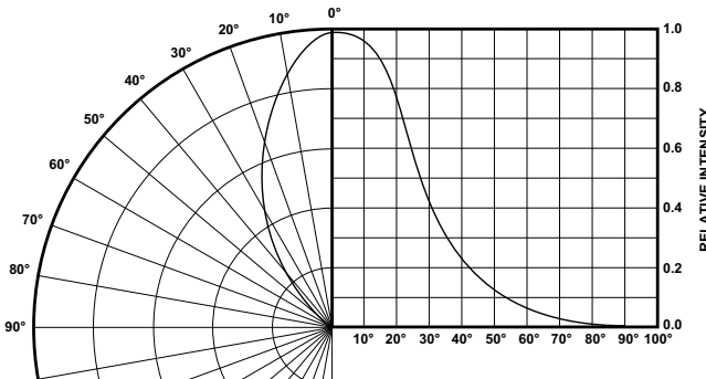
Figure 6: Relative Luminous Intensity vs. Angular Displacement for T-1 Lamp
