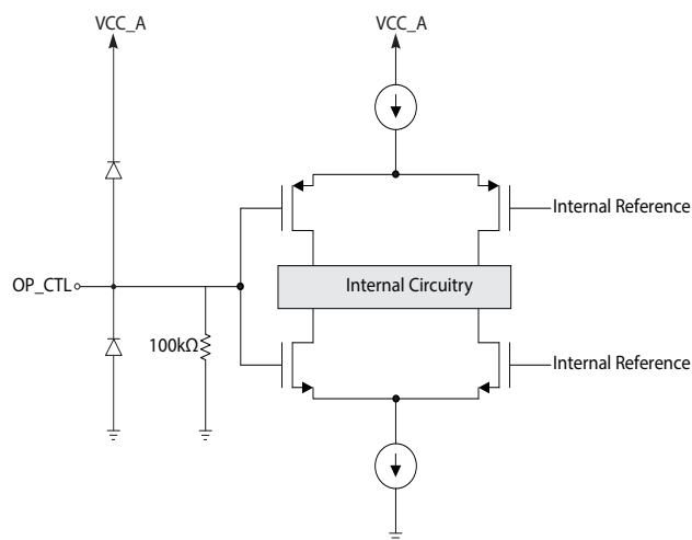
Figure 3-6: OP_CTL
