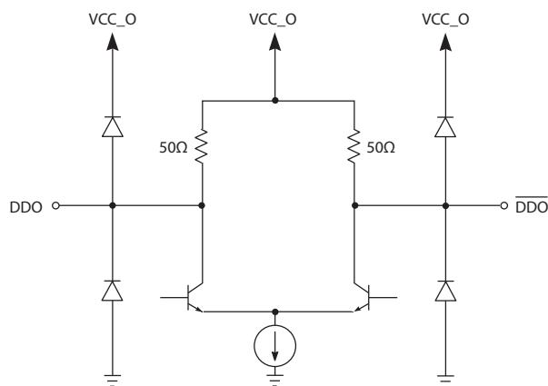
Figure 3-3: Output Circuit
