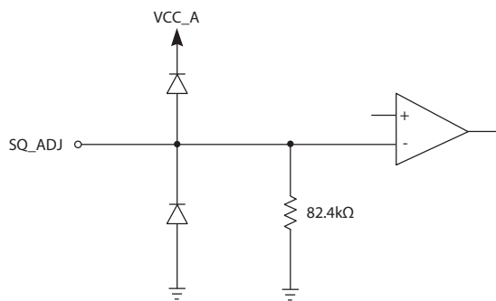
Figure 3-2: SQ_ADJ Circuit
