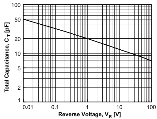
Figure 5. Total Capacitance
