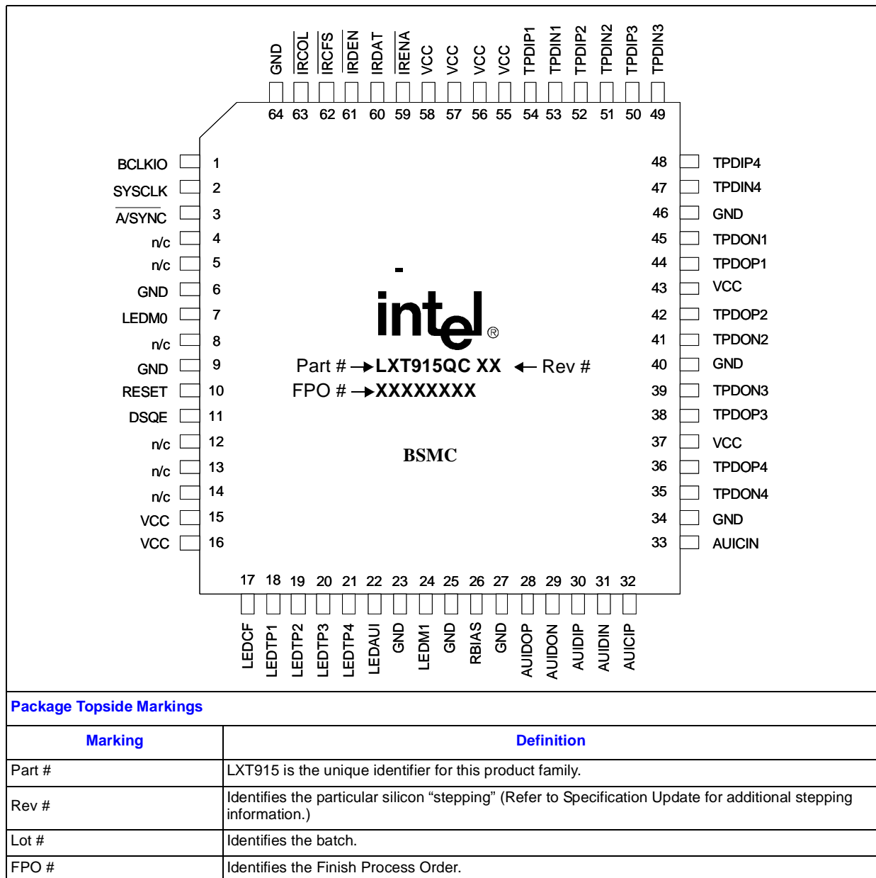
Figure 2. Pin Assignments
