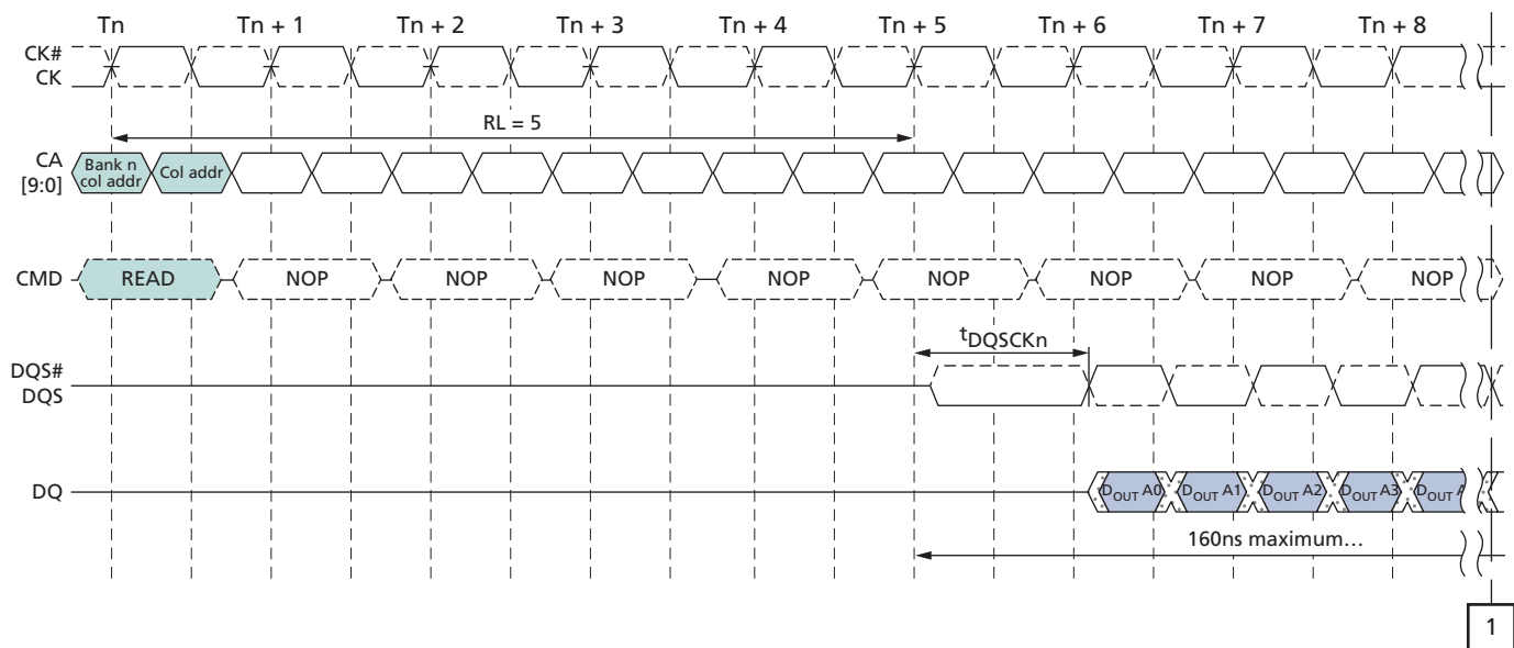
Figure 23: t_{DQSKDS} Timing
