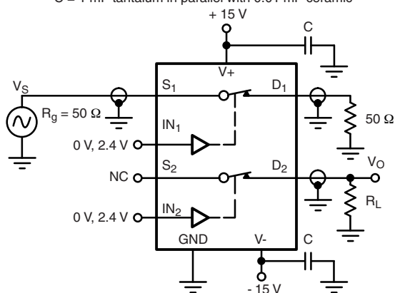
Figure 4. Crosstalk
