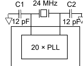
Figure 3. Crystal Configuration
