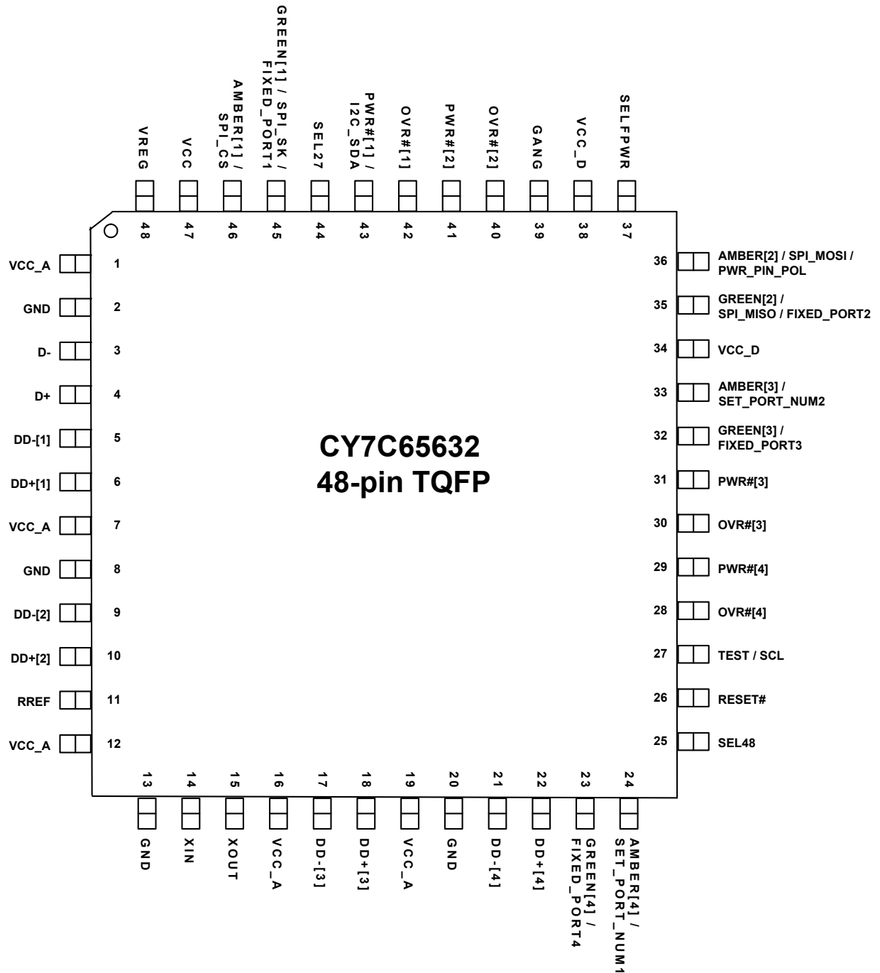
Figure 4. 48-pin TQFP (7 × 7 × 1.4 mm) pinout
