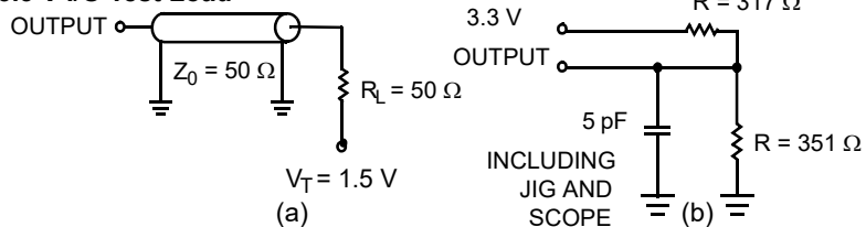
Figure 5. AC Test Loads and Waveforms
