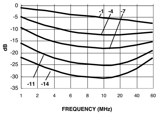
Attenuation CMS 1
