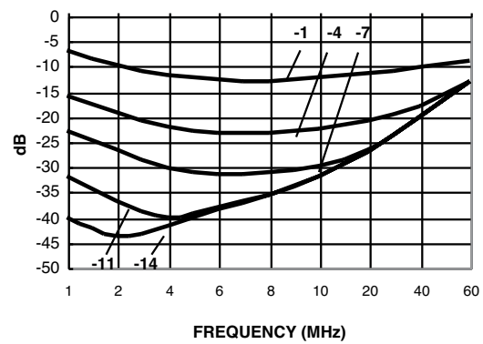
Attenuation CMS 2
