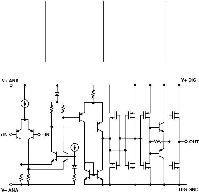
Figure 1. Simplified Schematic
