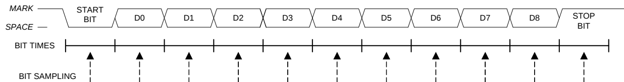
Figure 26.4. 9-Bit UART Timing Diagram
