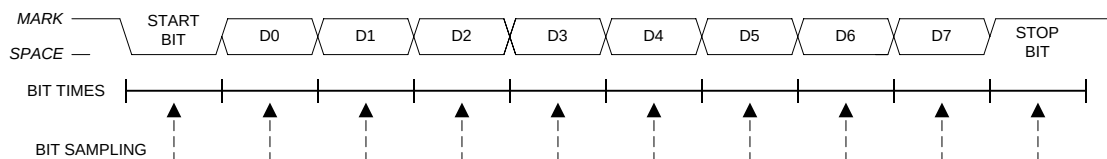
Figure 19.4. 8-Bit UART Timing Diagram
