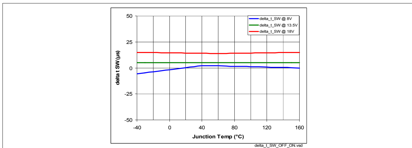
Figure 40 Turn ON / OFF matching \Delta t_{SW} = f(T_J; V_{GS}) , R_L = 12 \Omega
