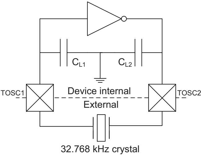
Figure 36-4. TOSC Input Capacitance
