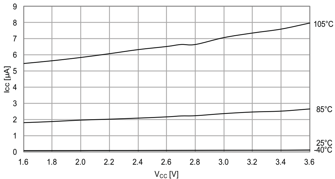
Figure 37-15. Power-down Mode Supply Current vs. V_{CC} All functions disabled.
