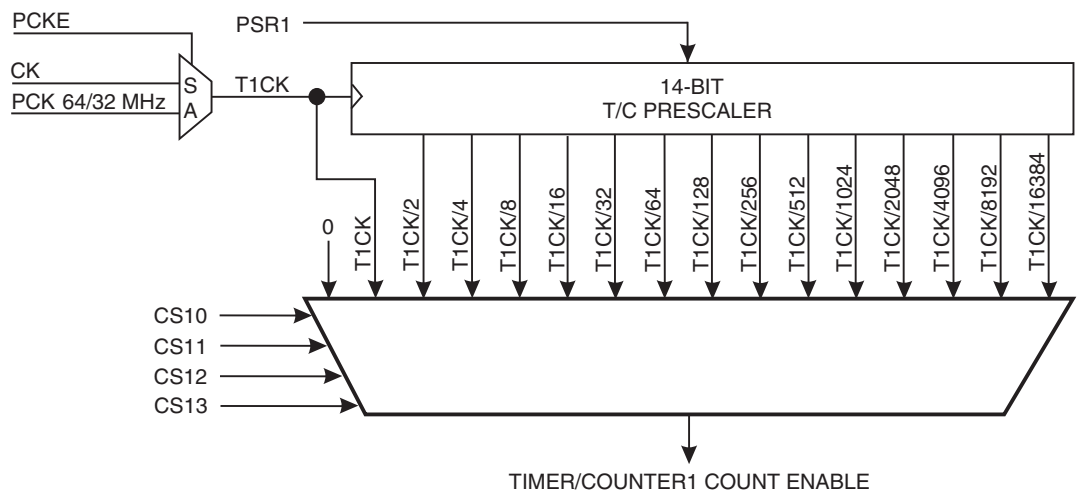
Figure 12-3. Timer/Counter1 Prescaler
