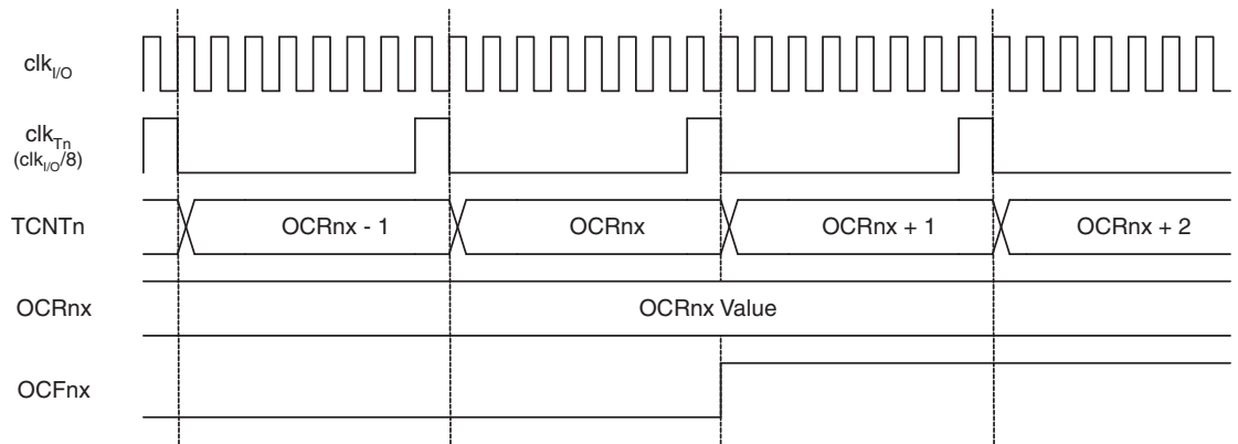
Figure 11-9. Timer/Counter Timing Diagram, Setting of OCF0x, with Prescaler ( f_{\text{clk\_I/O}}/8 )
