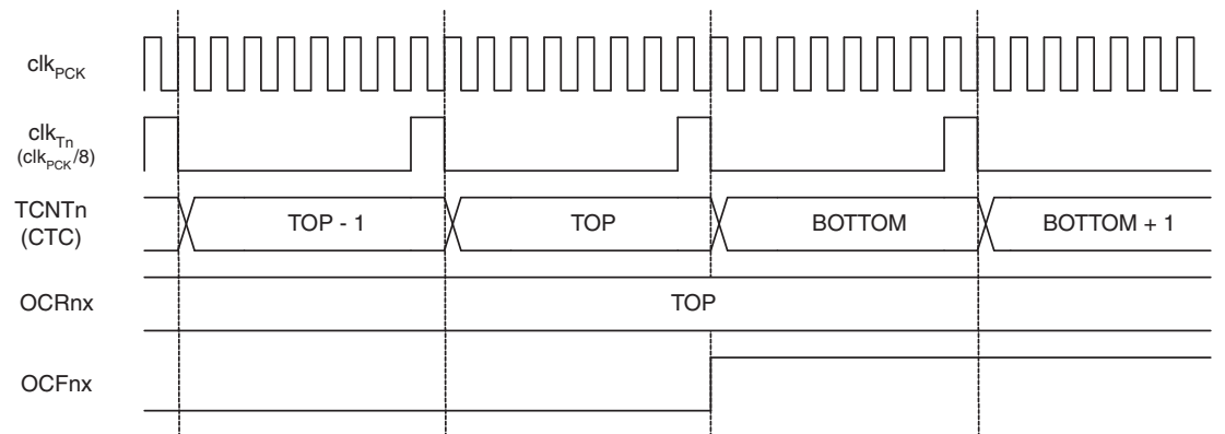
Figure 11-10. Timer/Counter Timing Diagram, CTC mode, with Prescaler ( f_{\text{clk\_I/O}}/8 )
