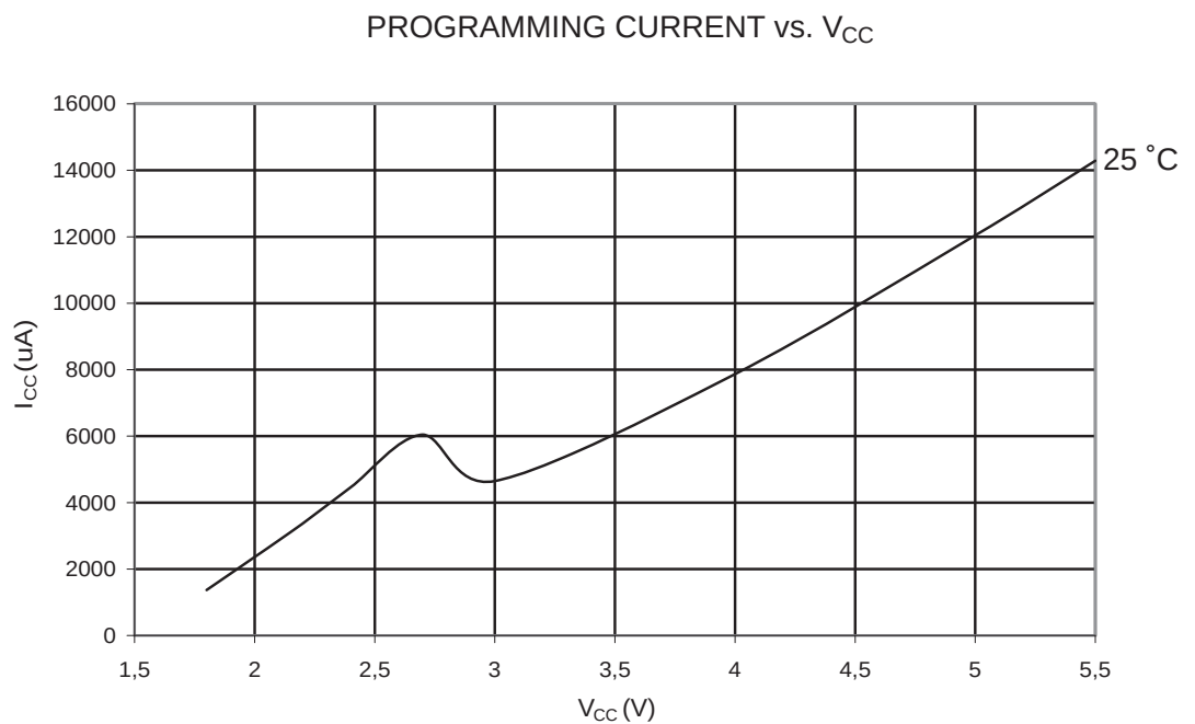
Figure 20-45. Programming Current vs. V_{CC}
