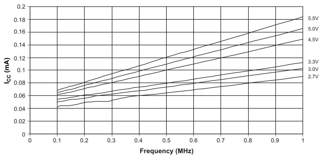
Figure 23-41. Reset Supply Current versus V_{CC} (0.1 to 1.0MHz, excluding Current Through the Reset Pull-up)
