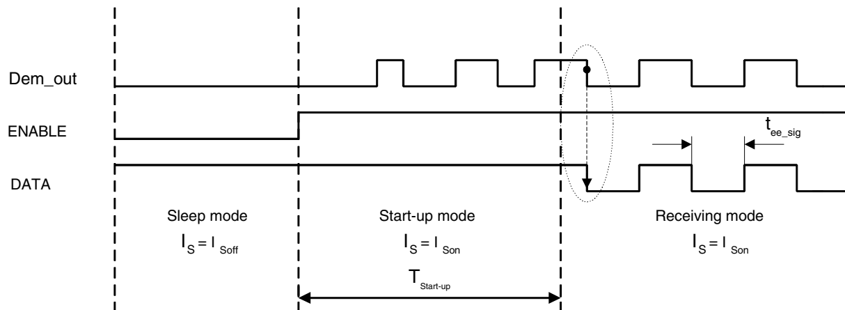
Figure 5-1. Enable Timing (1)
