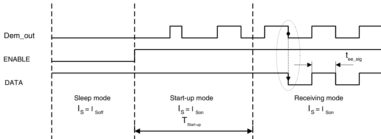
Figure 5-2. Enable Timing (2)
