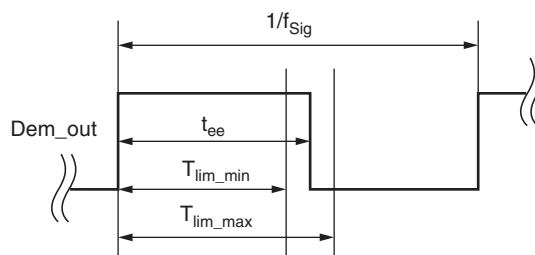
Figure 5-4. Valid Time Window for Bit Check
