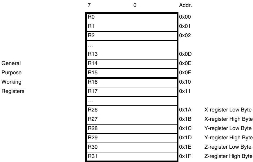
Figure 5-2. AVR CPU General Purpose Working Registers
