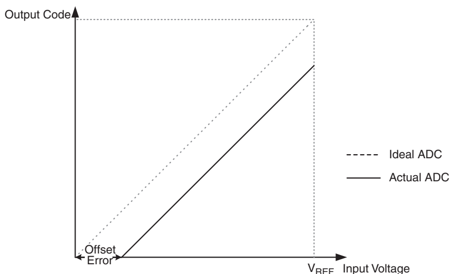
Figure 21-10. Offset Error
