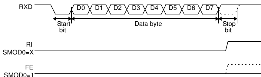
Figure 14-2. UART Timings in Mode 1
