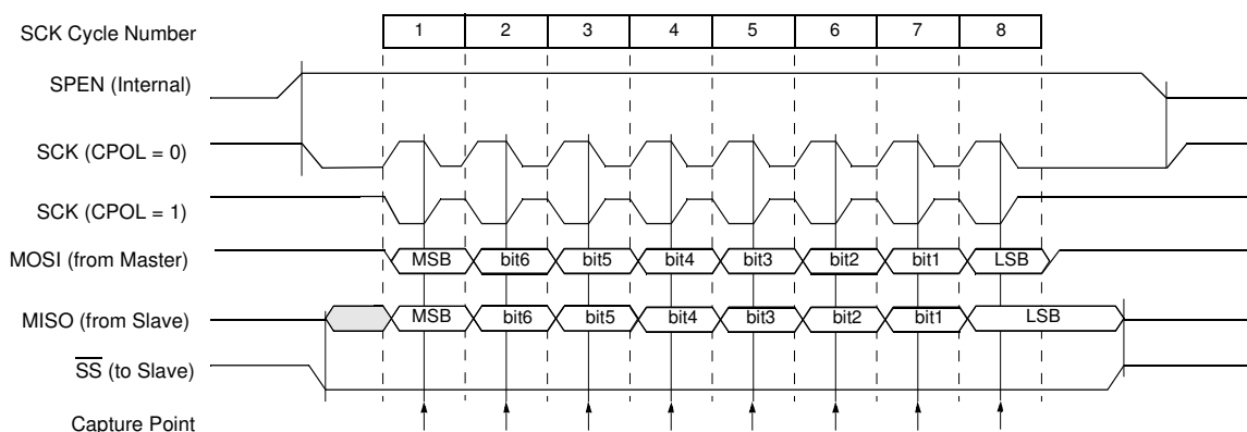
Figure 47. Data Transmission Format (CPHA = 1)
