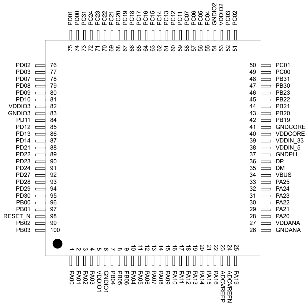
Figure 3-2. TQFP100 Pinout
