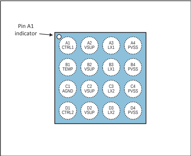
Figure 3: 16 Balls WL-CSP with 0.4mm Pitch
