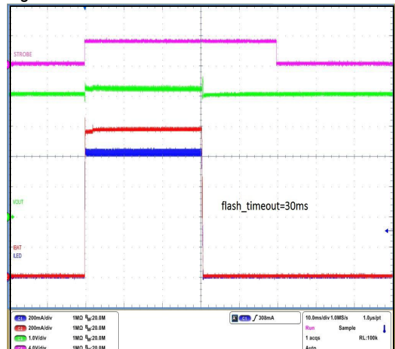
Figure 16. Flash Timeout
