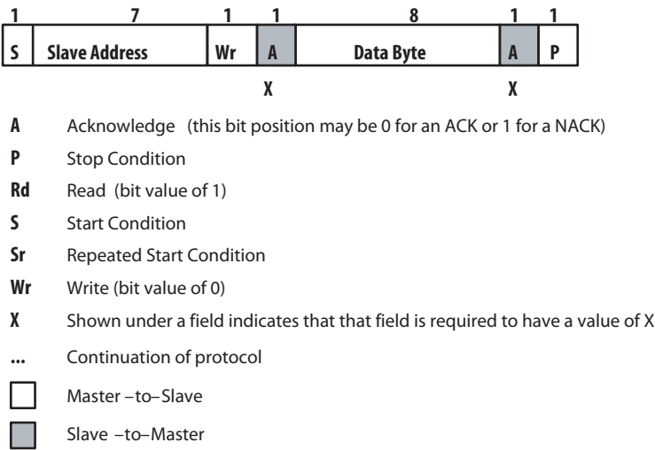
Figure 6. I²C Packet Protocol Element Key
