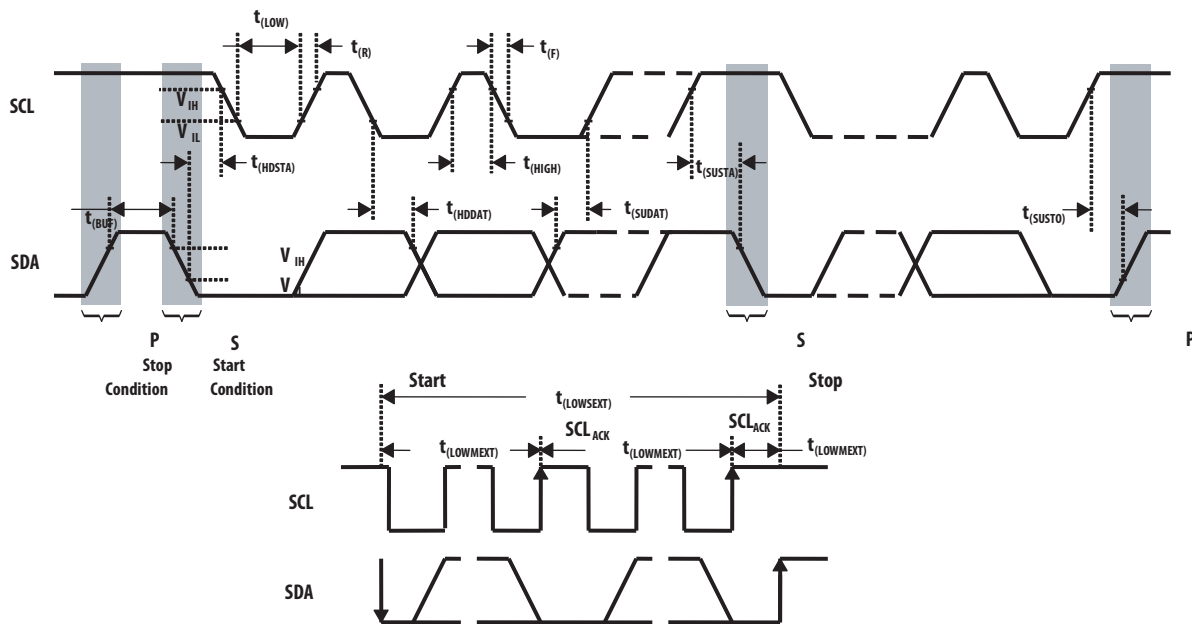
Figure 1. Timing Diagrams
