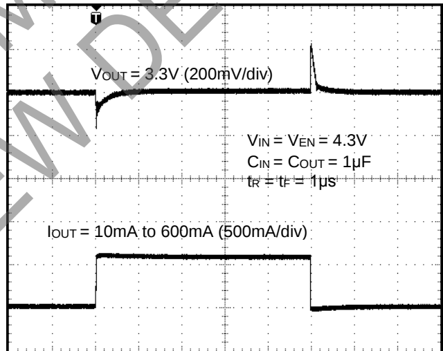
Load Transient Response Time (100μs/div)
