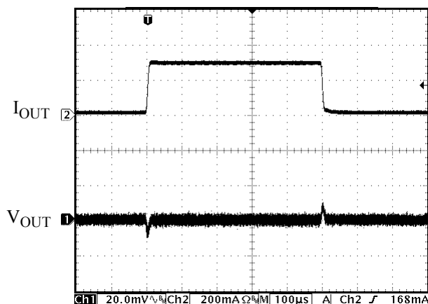
Figure 31. Load Transient (Conditions: C_{IN} = C_{OUT} = 1\mu\text{F} , V_{IN} = 2.5\text{V} , V_{OUT} = 0.8\text{V} , I_{OUT} = 10\text{mA} to 300\text{mA} )
