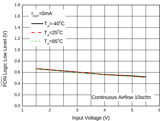
Figure 10. \overline{\text{FON}} Logic Low Level vs. Input Voltage
