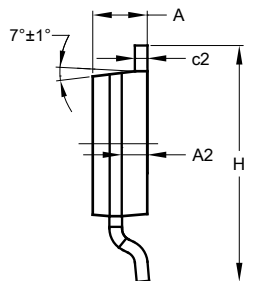
TO252-5
