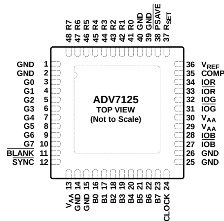
Figure 4. LFCSP Pin Configuration (CP-48-4)
