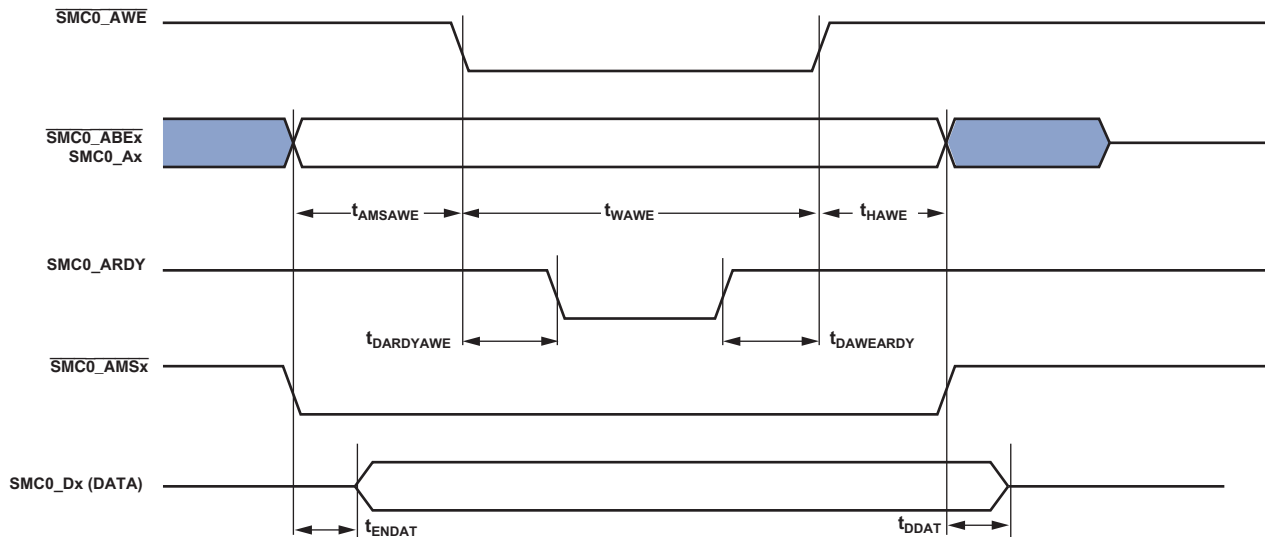
Figure 13. Asynchronous Write
