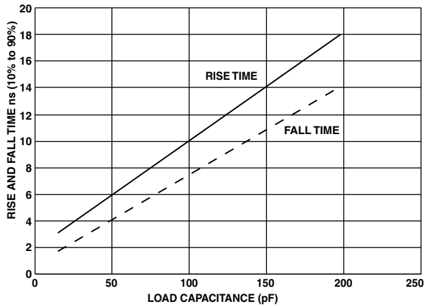
Figure 80. Typical Rise and Fall Times (10% to 90%) vs. Load Capacitance for Driver C at V_{DDEXT} = 3.65\text{ V}
