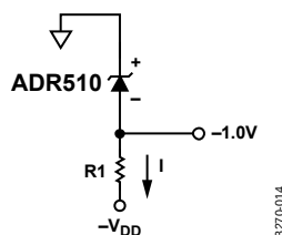
Figure 14. Precise -1.0\text{ V} Reference Configuration
