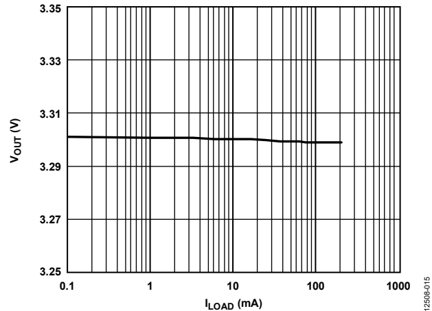
Figure 15. Output Voltage ( V_{OUT} ) vs. Load Current ( I_{LOAD} ), V_{OUT} = 3.3\text{ V}
