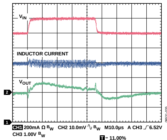
Figure 35. Line Transient, V_{OUT} = 5 V, PWM Mode, 800 mA, V_{IN1} = 6 V to 7 V, 2 µs Rise Time, C_{IN} = 3.3 µF
