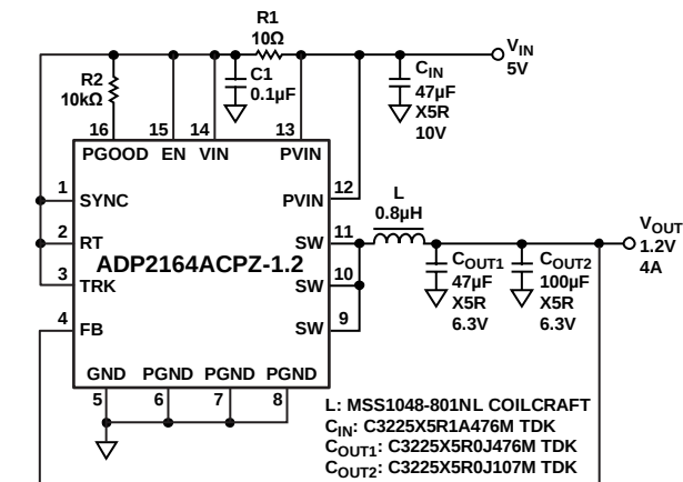
Figure 44. Fixed 1.2 V, 4 A, 1.2 MHz Step-Down Regulator
