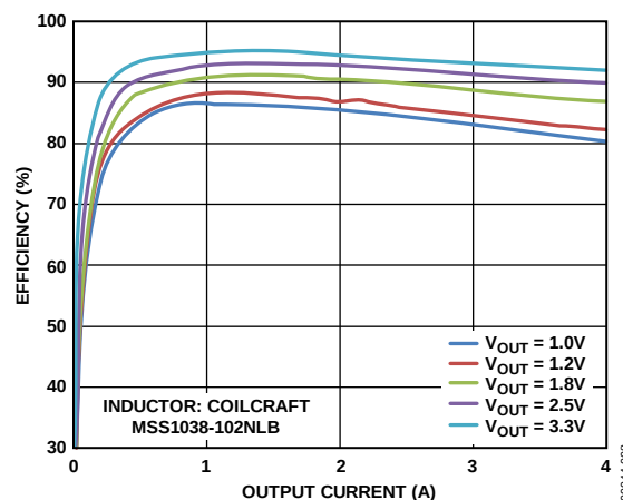
Figure 8. Efficiency vs. Output Current, V_{IN} = 5\text{ V} , f_S = 1.2\text{ MHz}
