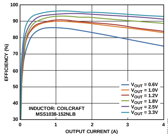
Figure 7. Efficiency vs. Output Current, V_{IN} = 5\text{ V} , f_S = 600\text{ kHz}
