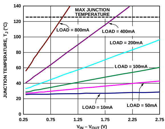
Figure 38. 0 mm² of PCB Copper, T_A = 25^\circ\text{C} , LFCSP
