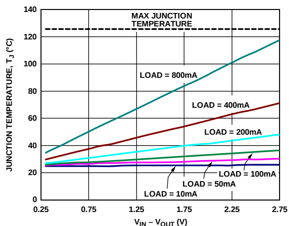
Figure 36. 6400 mm² of PCB Copper, T_A = 25^\circ\text{C} , LFCSP
