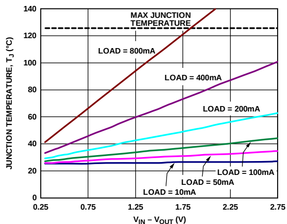
Figure 37. 500 mm² of PCB Copper, T_A = 25^\circ\text{C} , LFCSP
