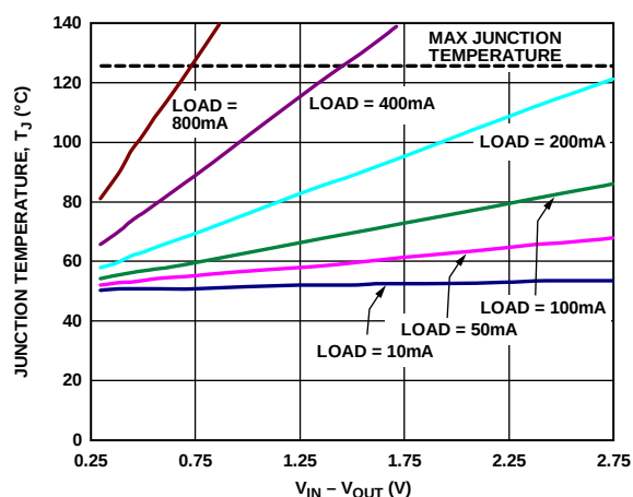
Figure 41. 0 mm² of PCB Copper, T_A = 50^\circ\text{C} , LFCSP
