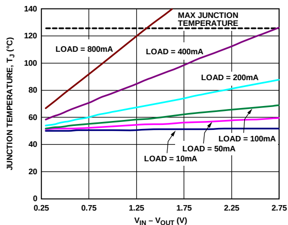
Figure 40. 500 mm² of PCB Copper, T_A = 50^\circ\text{C} , LFCSP
