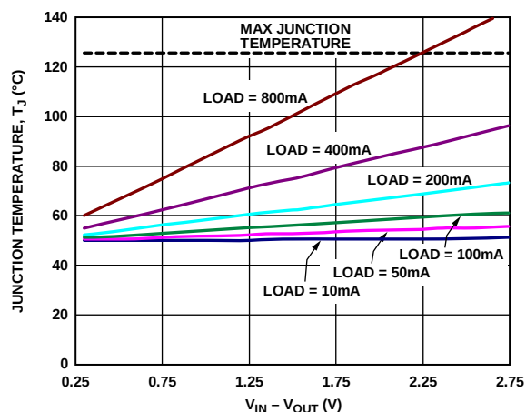
Figure 39. 6400 mm² of PCB Copper, T_A = 50^\circ\text{C} , LFCSP
