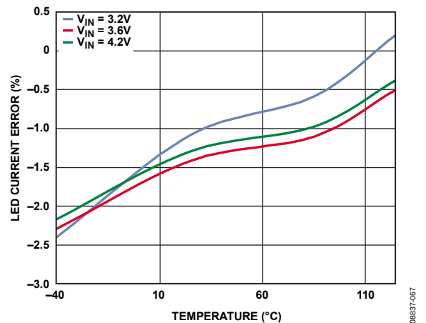
Figure 23. LED Current Accuracy vs. Temperature, I_{LED} = 800\text{ mA}
