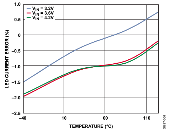
Figure 22. LED Current Accuracy vs. Temperature, I_{LED} = 1200\text{ mA}
