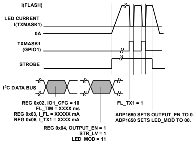
Figure 33. TxMASK1 Operation During Flash (Level-Sensitive) Mode
