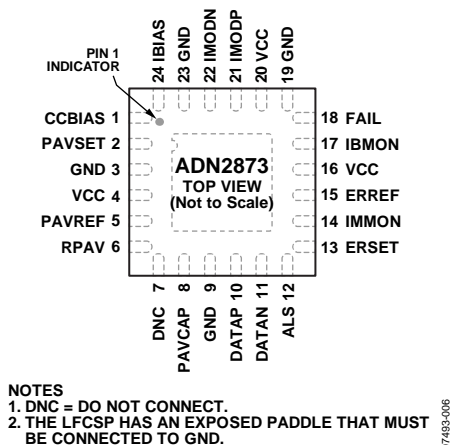
Figure 6. Pin Configuration
