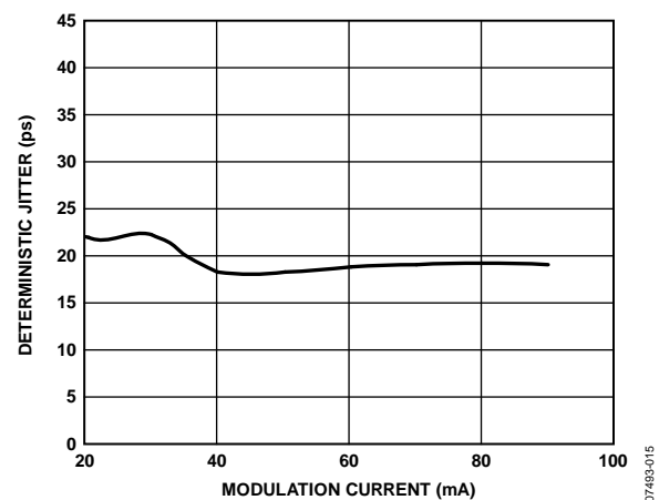
Figure 10. Deterministic Jitter at 2.488 Gbps vs. Modulation Current, I_{BIAS} = 20 mA
