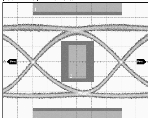
Figure 27. Optical Eye 2.488 Gbps, 65 ps/DIV, PRBS 2^{31}-1 P_{AV} = -0.2\text{ dBm} , ER = 8.96\text{ dB} , Mask Margin 21%, T_A = 85^\circ\text{C}
