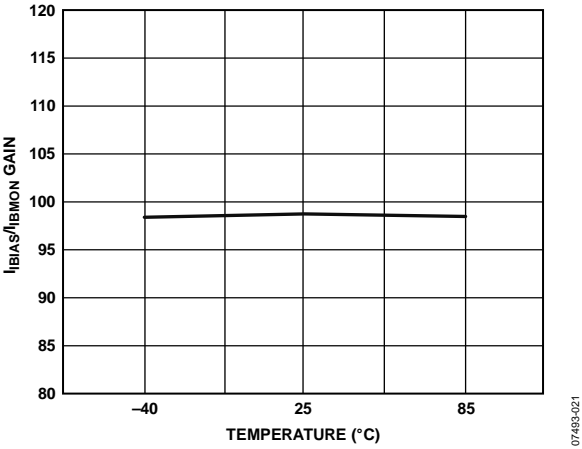
Figure 16. I_{BIAS}/I_{IMON} Gain vs. Temperature, I_{BIAS} = 11\text{ mA}
