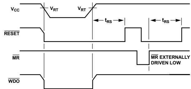
Figure 15. \overline{\text{RESET}} , \overline{\text{MR}} , and WDO Timing
