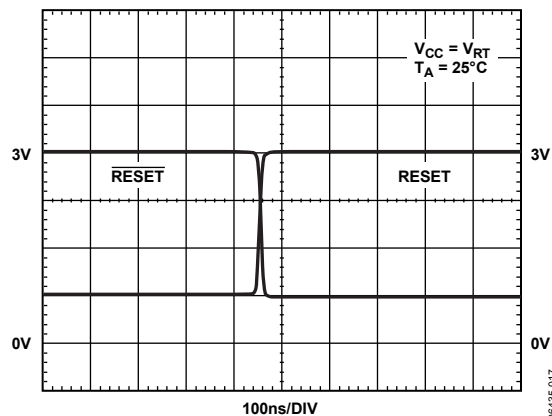
Figure 10. \overline{RESET} , RESET Assertion
