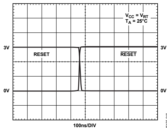
Figure 11. \overline{RESET} , RESET Deassertion
