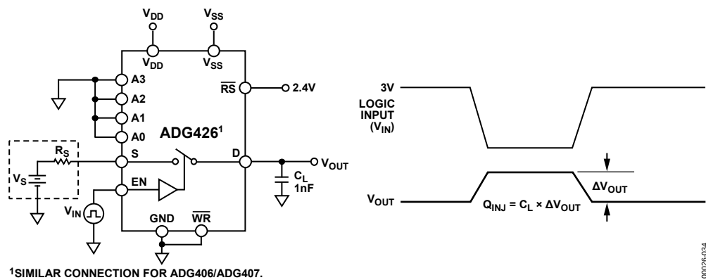
Figure 34. Charge Injection
