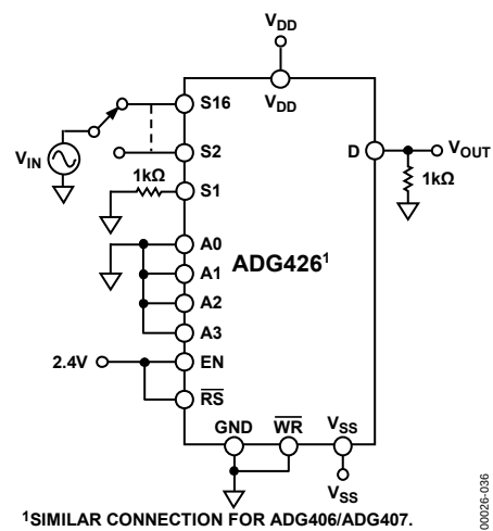
Figure 36. Crosstalk
