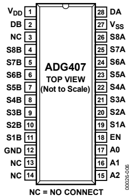
Figure 8. 28-Lead PDIP
