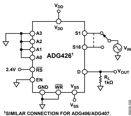
Figure 35. Off Isolation
