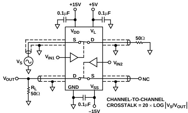
Figure 21. Channel-to-Channel Crosstalk
