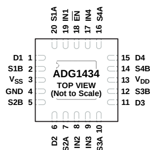
Figure 7. ADG1434 LFCSP Pin Configuration
