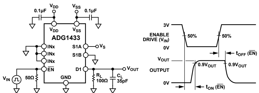
Figure 30. Enable Delay, t_{ON}(\overline{EN}) , t_{OFF}(\overline{EN})
