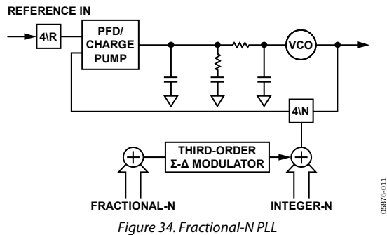
Figure 34. Fractional-N PLL
