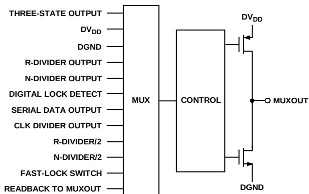
Figure 20. MUXOUT Schematic
