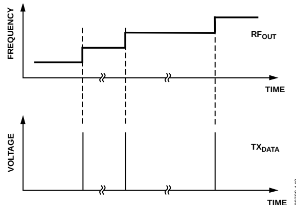
Figure 42. External Control of Ramp Steps
