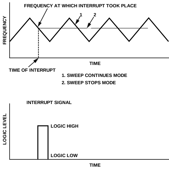
Figure 43. Interrupt and Frequency Readback
