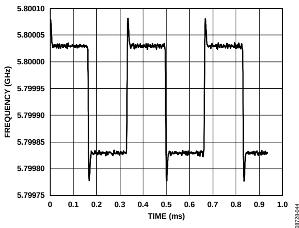
Figure 13. FSK; Settings: Frequency Deviation = 100 kHz, Data Rate = 3 kHz
