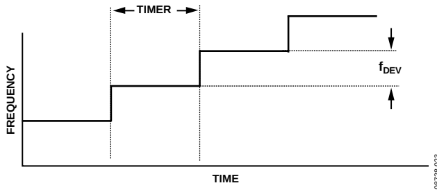
Figure 35. Waveform Timing
