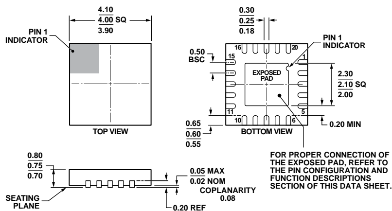
Figure 27. 20-Lead Lead Frame Chip Scale Package [LFCS_P_WQ] 4 mm × 4 mm Body, Very Very Thin Quad (CP-20-6)
